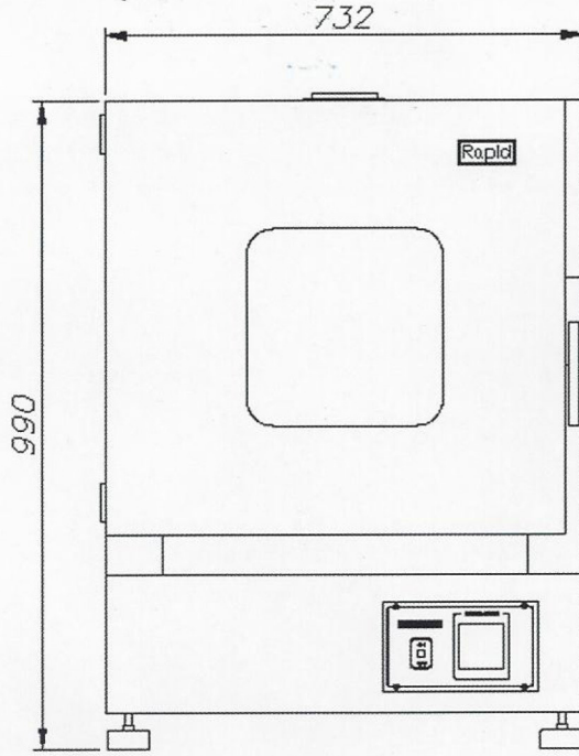
FRONT (正視圖)
